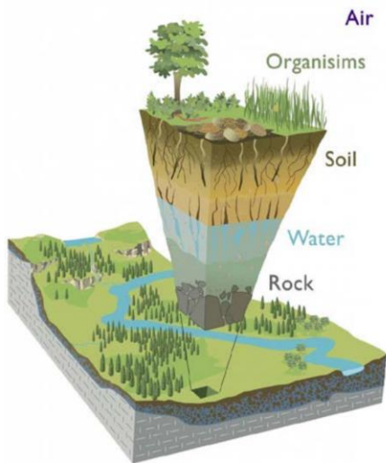
The Critical Zone is Earth's outer skin NRC & CZO, 2014
