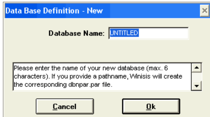
Figure 50 - Database > New
