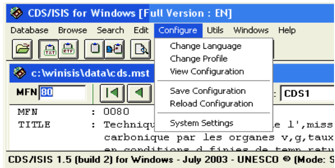
Figure 17 - Configure Menu
