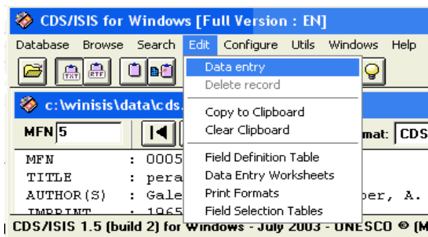
Figure 12 - Edit Menu
