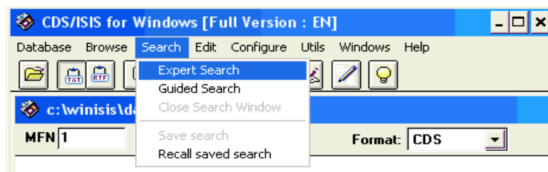
Figure 11 - Search Menu
